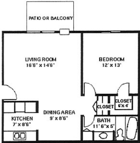
ONE BEDROOM 696 Sq. Ft.
