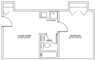
COLONIAL TERRACE 1 BEDROOM
